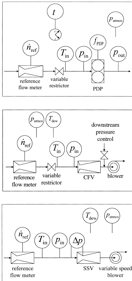
Figure 1 of 1065.340 CVS calibration configurations.
